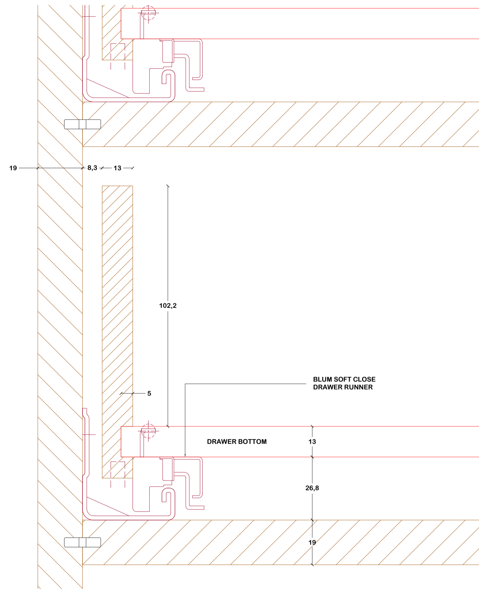
DRAWER RUNNER DETAIL 1:1
