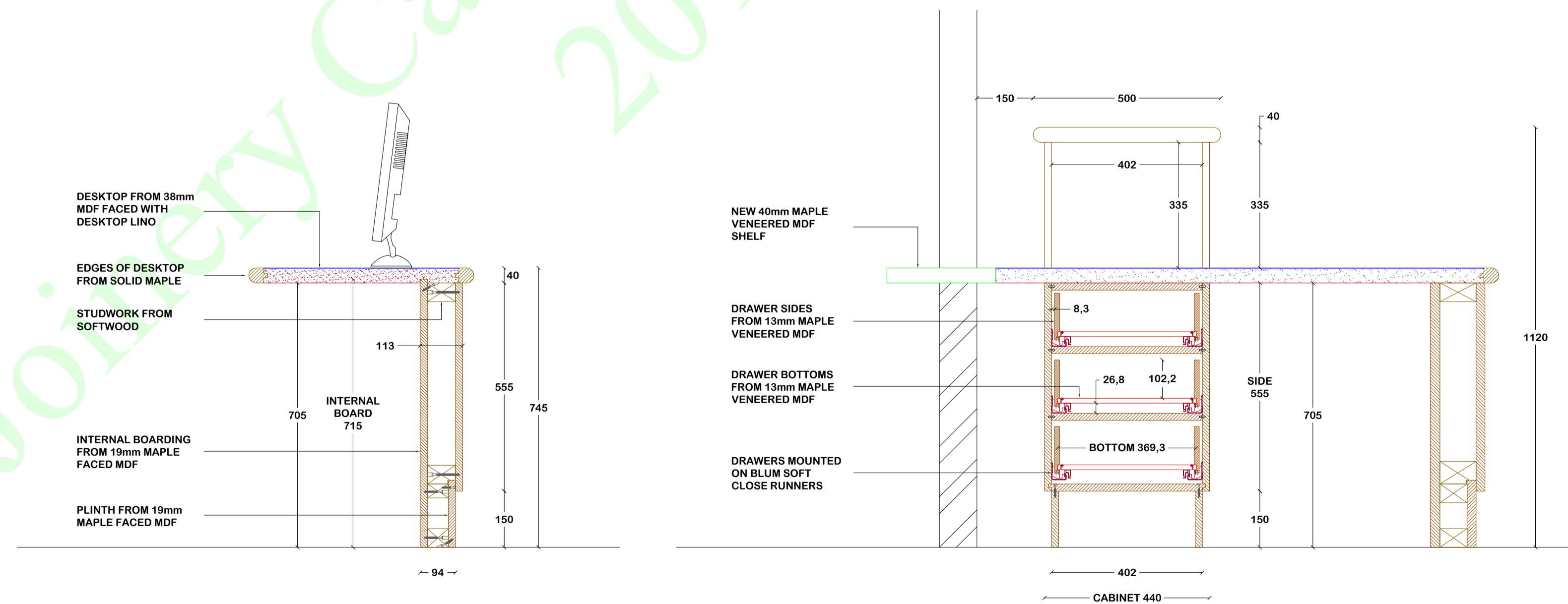
SECTION 03 DETAIL 1:10
