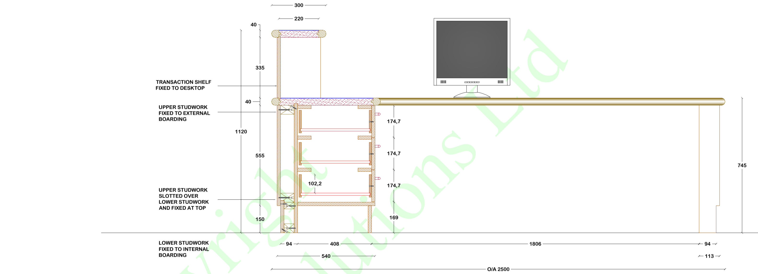
SECTION 02 DETAIL 1:10
