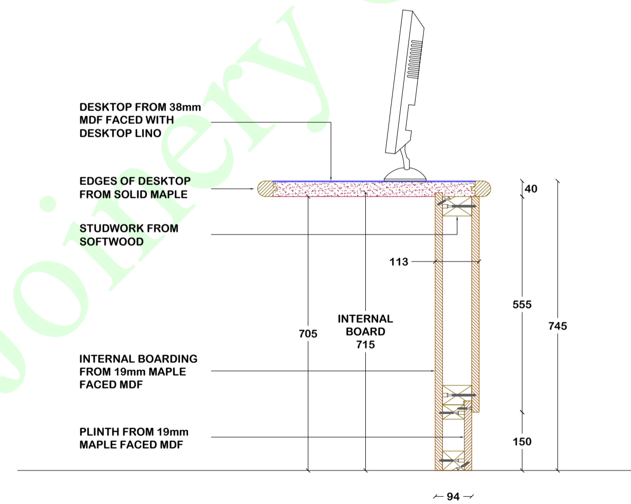
SECTION 01 DETAIL 1:10
