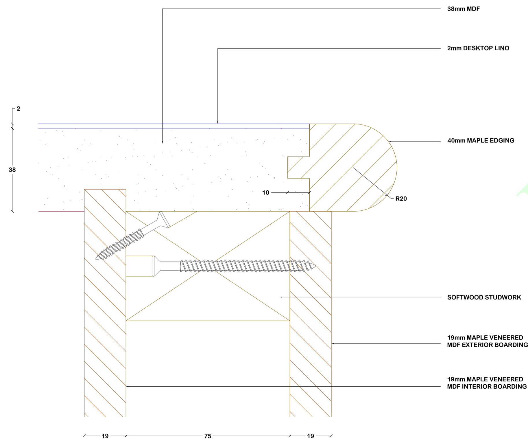
DESKTOP DETAIL 1:1
