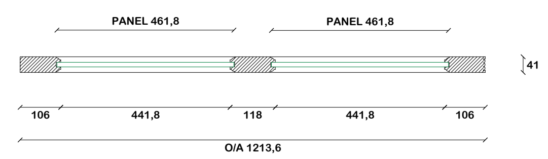
SECTION 01 DETAIL 1:10
